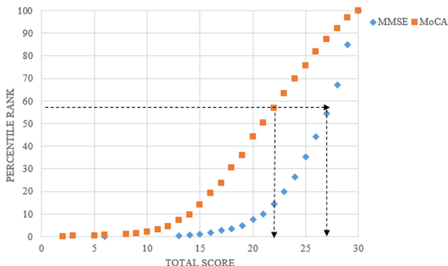
FIGURE 2 Equipercile equating in MoCA and MMSE values in 803 patients from the Memory Clinic FELIX PLATTER, Switzerland. MMSE values are given in raw values. MoCA values correspond to education-adjusted values. The dotted lines indicate that MoCA and MMSE values are set equal when their corresponding percentile ranks are equal. MMSE, mini mental status examination; MoCA, montreal cognitive assessment.
